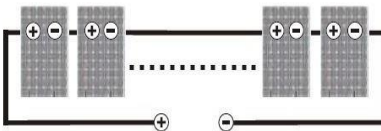
Fig: Series connection for more Voltage
