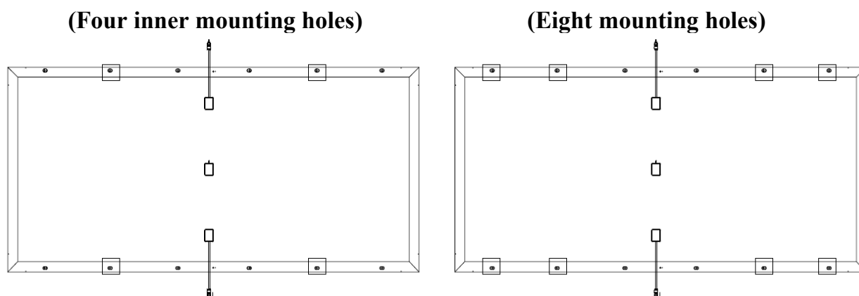
Fig: Mounting Details-2
