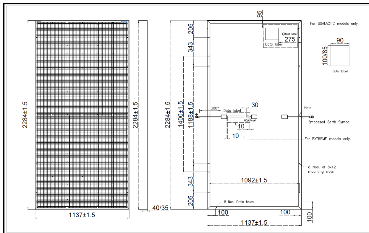
Fig: Finished Module Details (For Reference only)
