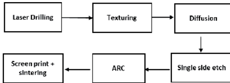
Figure 7. Process flow of MWT PERC solar cells.
