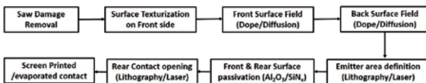
Figure 8. IBC process flow.
